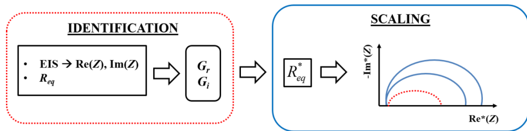
Figure 1 – Scheme of the proposed scaling-up methodology procedure.
