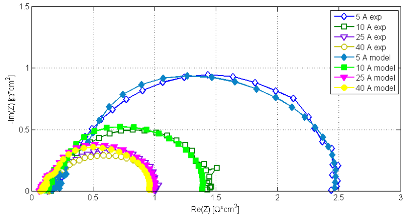
Figure 3 – Results in PEMFC impedance prediction at different operating currents (D-CODE data [18]). The experimental data are depicted with empty markers, whereas model results are depicted with filled markers.
