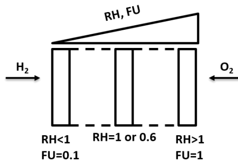
Figure 2 – Hypothesis adopted for RH and FU distribution along the stack.
