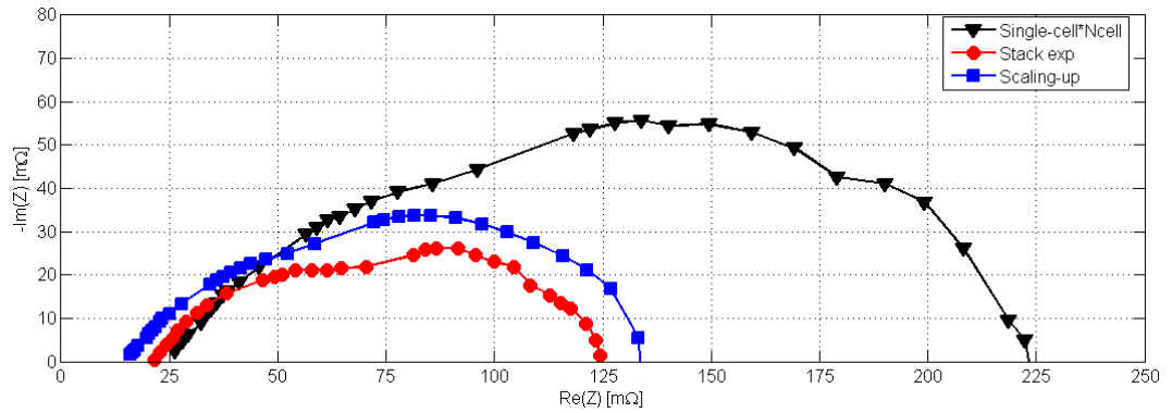
Figure 7 – Comparison of stack measured impedance (●) with the simple multiplication of the stack last-cell impedance times the number of cells (▼) and the spectrum resulting scaling the stack last-cell impedance to obtain the full-stack impedance with the proposed methodology (■).
