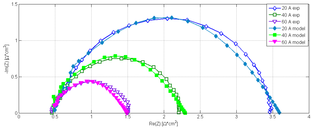
Figure 4 – Results in PEMFC impedance prediction at different operating currents (Asghari data [19]). The experimental data are depicted with empty markers, whereas model results are depicted with filled markers.
