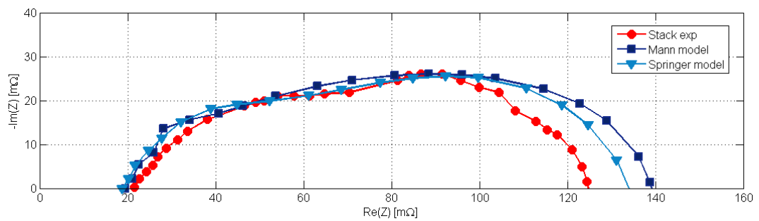
Figure 6 – Comparison of stack measured impedance (●) with the proposed methodology results by using the models of Mann (■) and Springer (▼), respectively.
