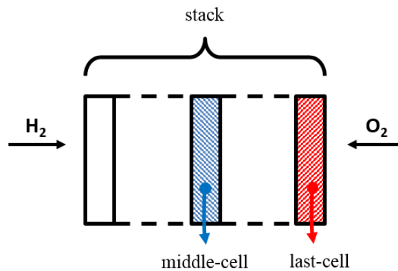
Figure 5 – Schematic visualization of the cells, which were selected for identifying non dimensional parameters in the two analysis presented in sections 3.2.1. and 3.2.2.
