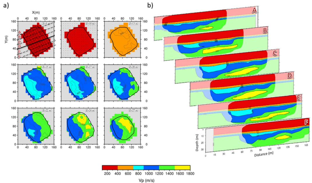
Figure 3. P-wave velocity model. (a) Horizontal slice of P-wave velocity model at different depths. The black contour delimitates the resolved area, i.e. the area for which the three resolution parameters (RDE, S j and DWS) are included in a threshold value. The threshold values of S j and DWS are chosen in order to obtain a similar contour, binding the RDE to be higher than 0.9. The grey regions in each slice represent areas not covered by rays. (b) P-wave velocity model projected onto the SW-NE cross-sections located in Fig. 3a. The blurred regions in each slice represent areas not resolved.
