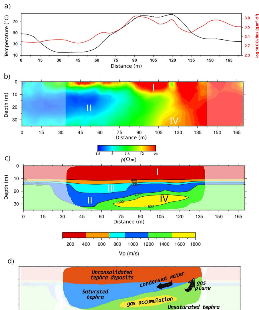
Figure 4. Comparison between temperature (black line) and CO 2 flux (red line) in (a), resistivity cross section in (b) and P-wave velocity model projected onto the cross-section D in Fig. 3a in (c). (d) Schematic representation of geological features and fluid flux direction, discussed in the interpretation.
