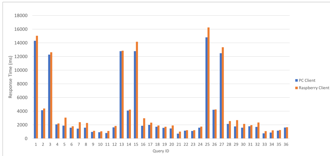
FIGURE 2 Response times comparison between PC based client and Raspberry based client for each performed query.
