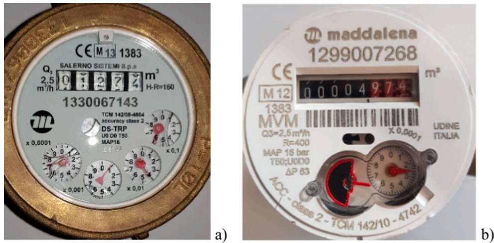
Fig. 5. The analyzed meters (a) multijet and (b) volumetric rotary piston.
