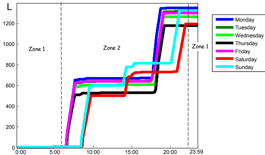
Fig. 1. Daily consumption curves concerning a week.
