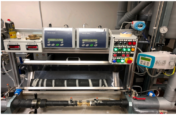
Fig. 3. The characterization station of the “LAMI” Laboratory.
