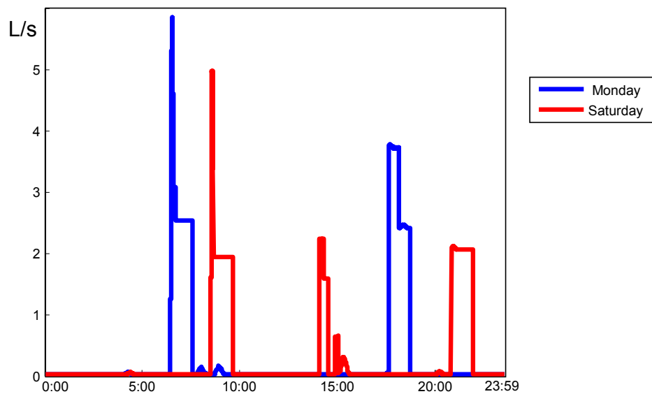
Fig. 2. Daily flow rate monitoring for two days of the week.
