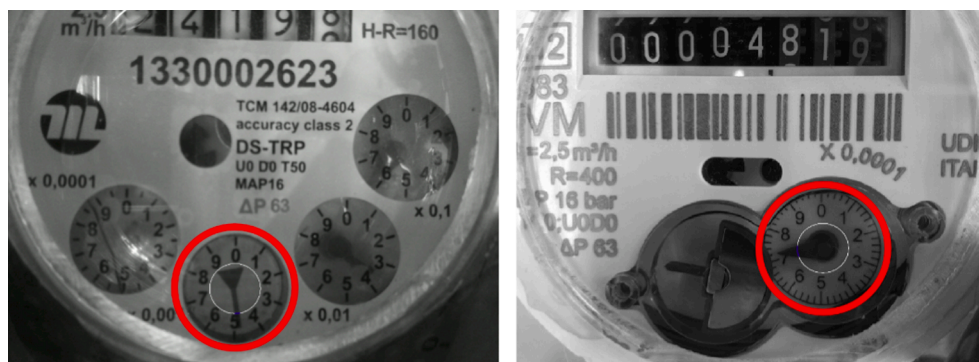
Fig. 8. Needles highlighted in red with the circumference locus of points in white and intersection with the indicator in blue. (a) multijet water meter, and (b) volumetric rotary piston water meter.
