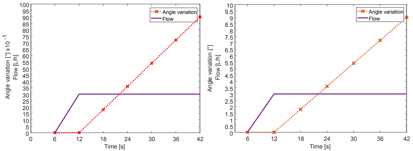
Fig. 9. Angle variation in red, with flow profile in blue. (a) multijet water meter, and (b) volumetric rotary piston water meter.
