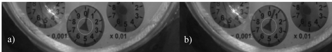
Fig. 10. Acquired image at the start of the test (a) and the end of test (b) for the multijet water meter.
