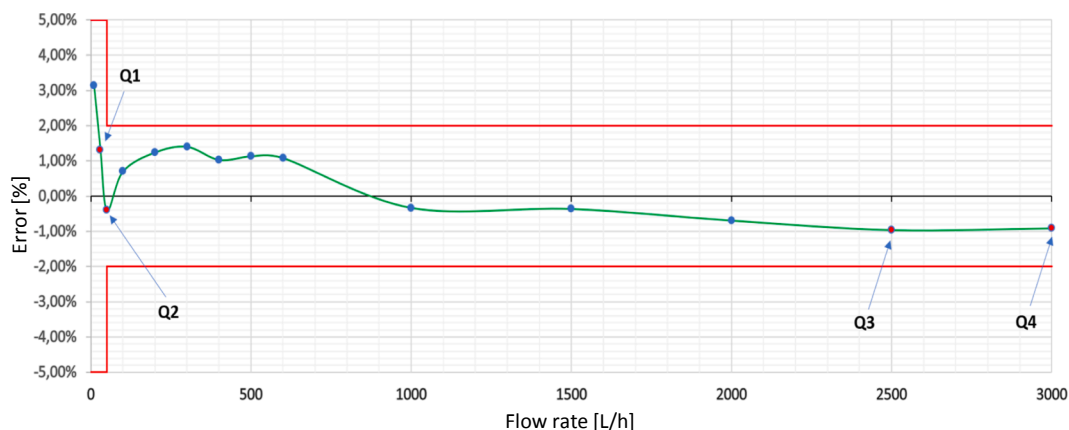
Fig. 4. Experimental results of the ultrasonic sensor hydraulic characterization. The red lines represent the maximum tolerated relative error.
