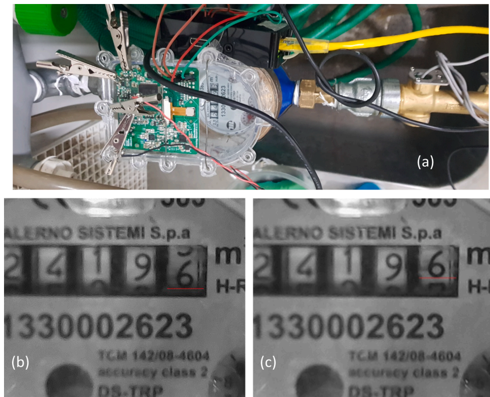
Fig. 6. TH evaluation for the multijet meter, (a) the connection of the meters to the characterization station, (b) acquired image at the start of test (c) acquired image at the end of the test.
