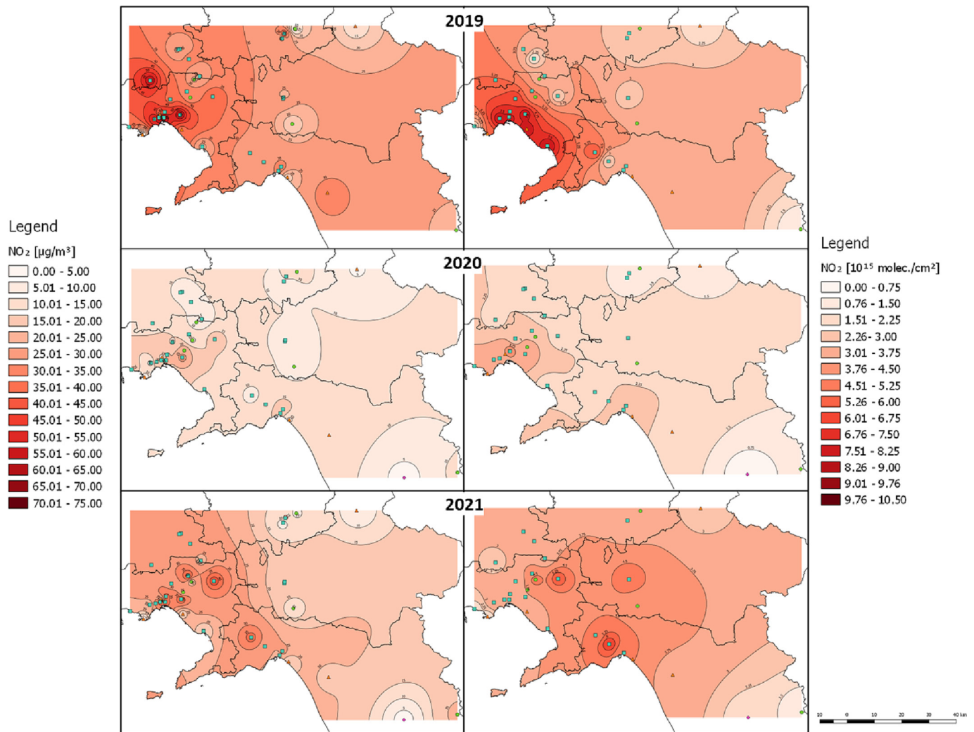
Fig. 6. Comparison between the interpolation of NO 2 ground level concentration (left) and of NO 2 tropospheric column concentration (right), for the selected days (30th March 2019, 7th April 2020, 11th March 2021).
