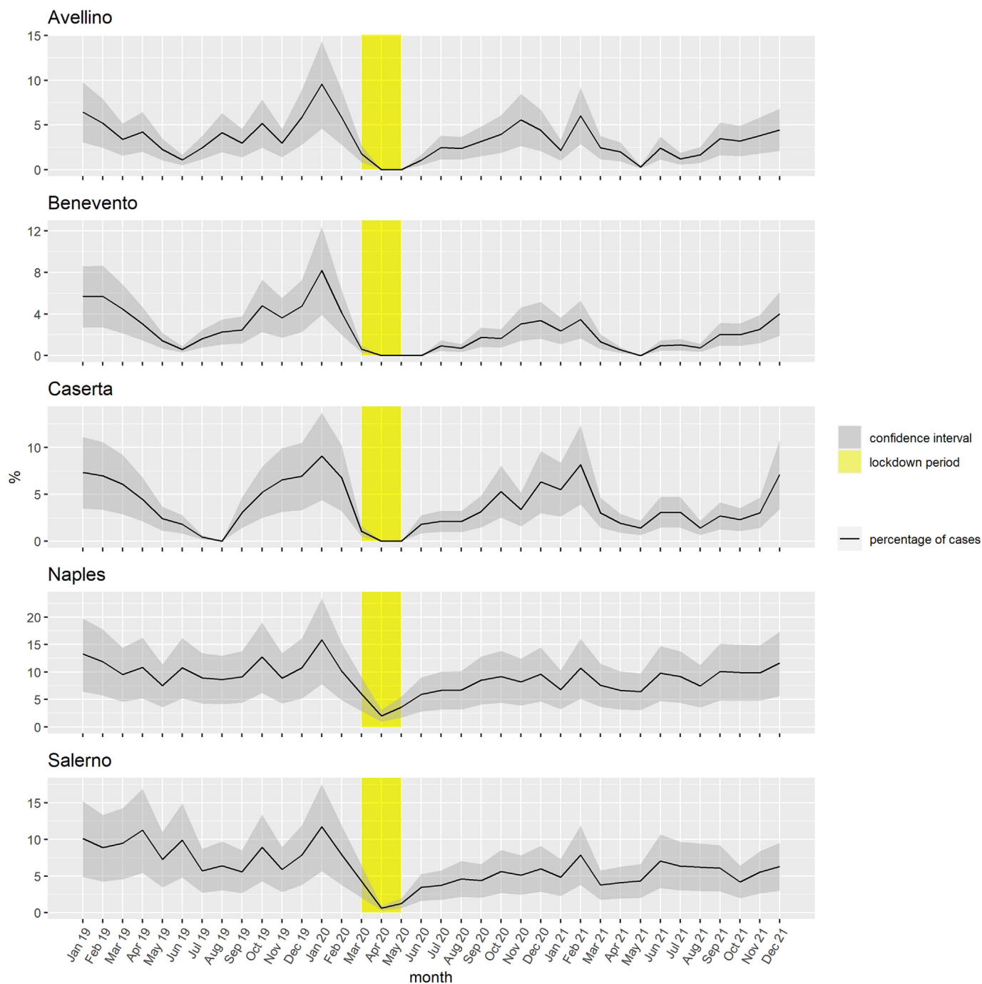
Fig. 5. Estimated proportion of deaths in adults (age 30 + ) attributable to \text{NO}_2 concentration. Lockdown period is highlighted in yellow; the grey area is the 95 % confidence interval. (For interpretation of the references to colour in this figure legend, the reader is referred to the web version of this article.)
