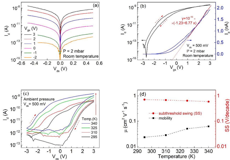
Fig. 2. (a) Output characteristics for different V gs . (b) Transfer characteristics at V ds = 500 mV and pressure of 2 mbar for a forward and a reverse V gs sweep, on logarithmic (black) and linear (blue) scale. (c) Transfer characteristics at V ds = 500 mV, ambient pressure, and for different temperatures. (d) Mobility (black) and subthreshold swing SS (red) as a function of temperature. All measurements are performed in dark.
