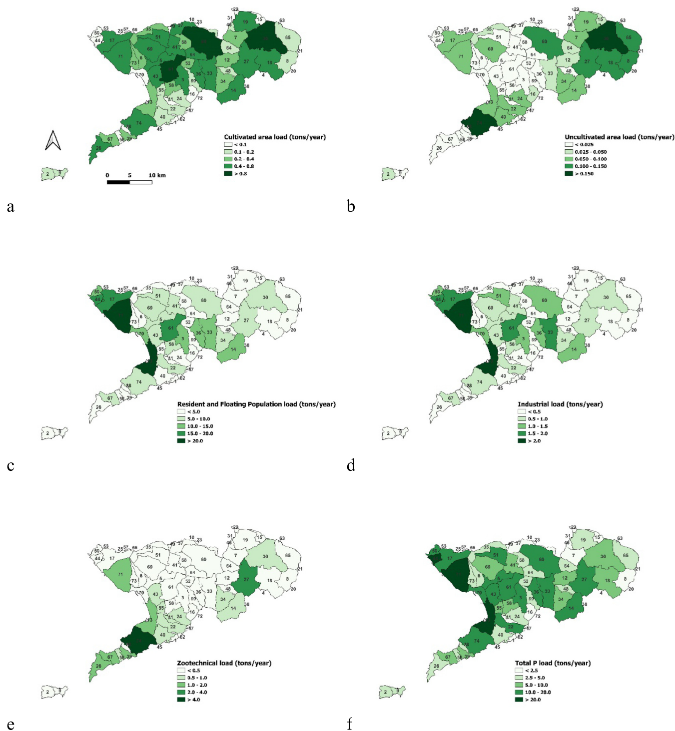
Fig. 10. Spatial distribution of phosphorous load per each municipality belonging to UoM-Sarno. a) Cultivated area load; b) Uncultivated area load; c) Resident and floating population load; d) Industrial load; e) Zootechnical load; and f) Total phosphorous pollution load.
