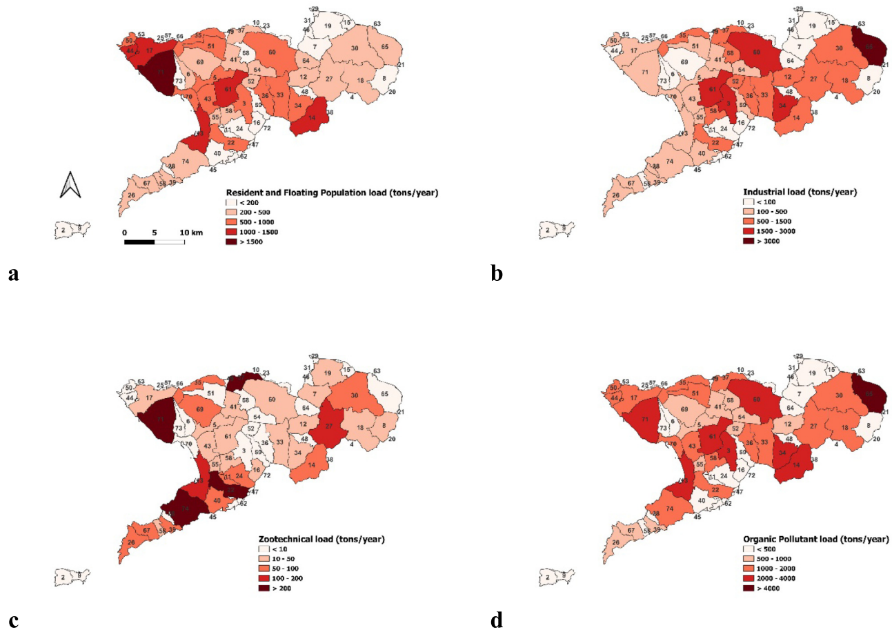
Fig. 7. Spatial distribution of OPL per each municipality belonging to UoM-Sarno (referred to 2018 data); a) Resident and Floating population load; b); Industrial load; c) Zootechnical load; and d) Total organic polluting load.
