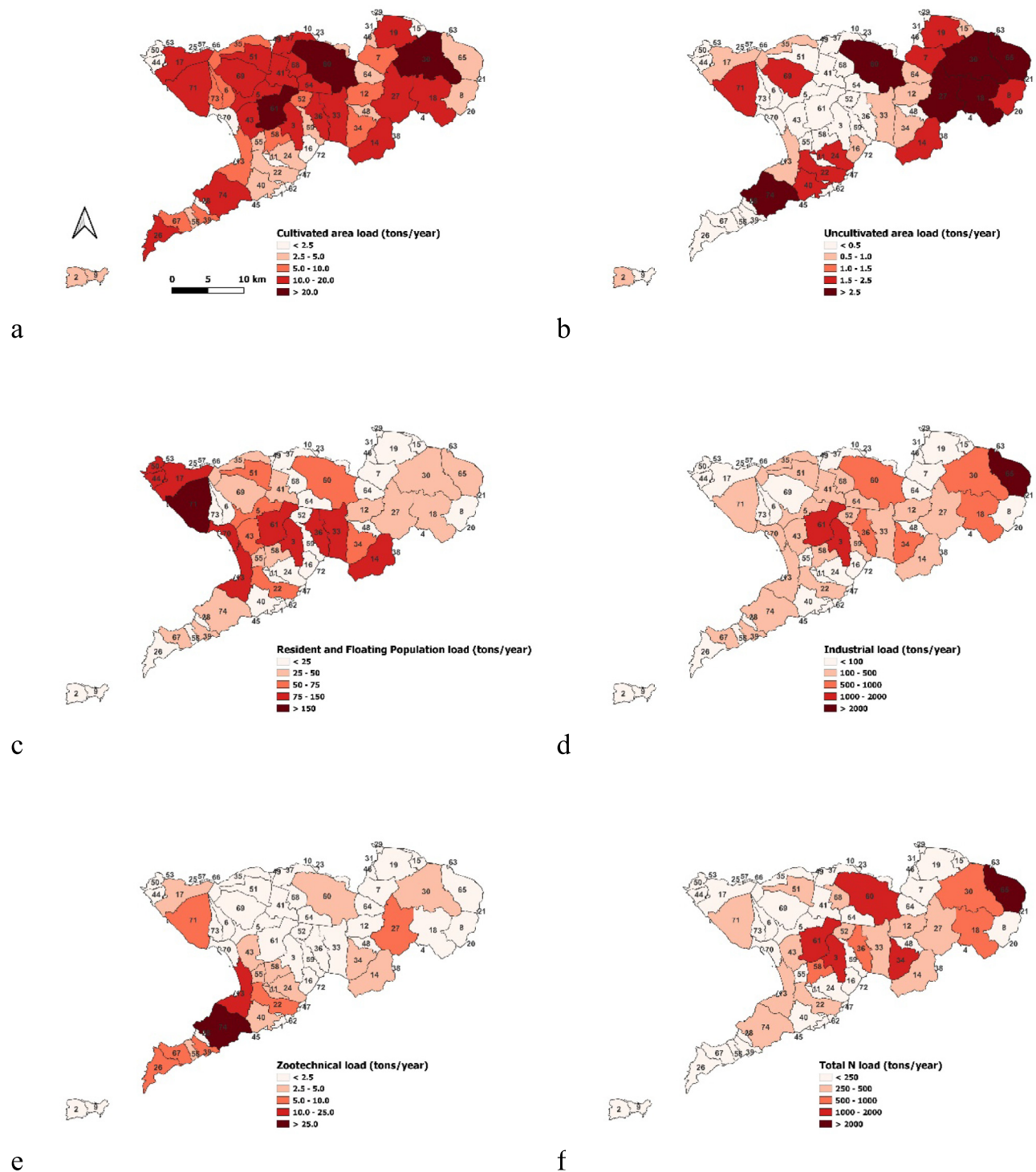
Fig. 9. Spatial distribution of nitrogen load per each municipality belonging to UoM-Sarno. a) Cultivated area load; b) Uncultivated area load; c) Resident and floating population load; d) Industrial load e) Zootechnical load; and f) Total nitrogen pollution load.
