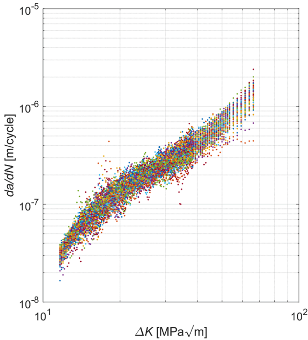
Fig. 3. FCG material data for aluminium alloy 2024-T3. [15,50].
