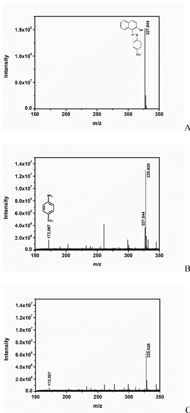
Fig. 6. ESI-MS spectra on (A) untreated AO7(20 mg/L); (B) 1 min of UV/ZVI-ZnS (1 g/L), (C) 160 min of UV/ZVI-ZnS (1 g/L).
