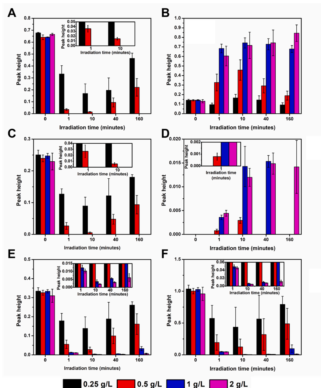
Fig. 4. – Change of absorbance values at 230 nm (A), 250 nm (B), 308 nm (C), 345 nm (D), 403 nm (E) and 484 nm (F) versus time e for different concentrations of ZVI-ZnS under UV-A radiation. When present, the insets show a magnification of the plots.
