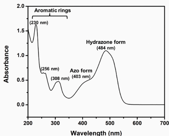
Fig. 1. UV-Vis absorbance spectrum of AO7 solution (20 mg/L).
