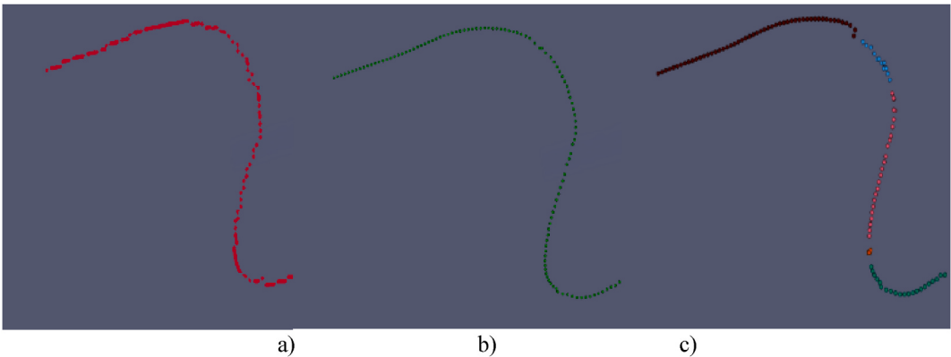
Fig. 13. Representative image of the central axis smoothing result obtained. In a), the original central axis referred to a vessel; in b) the smoothing result obtained downstream of the optimization process of the Delta and Threshold parameters; in c) the result in the worst case where the same portion of the vessel is the result of several strokes together.
