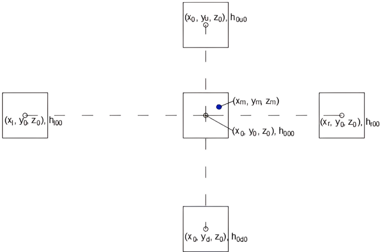
Fig. 8. Depiction scheme of the central axis smoothing procedure described. The original central point coordinates located at the center of the relative voxel, marked by the empty circle, are recomputed throughout a weighted average evaluation of the adjacent voxels of the vessel's cross section belonging area, along the horizontal and vertical directions. The procedure reiterates for all the three cross sections centered in the considered point. The algorithm returns the new x, y, and z coordinates of the central point, highlighted in the filled circle.
