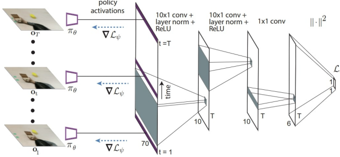
Figure 3.4: The Temporal Adaptation Loss architecture applies 1D temporal convolutional layers to the stacked embeddings generated by the policy \pi from the frames of the human video demonstration.
