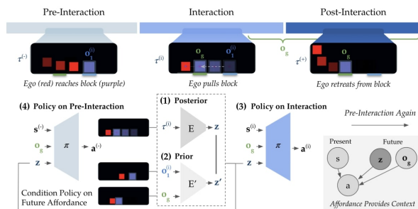
Figure 2.6: PLATO architecture proposed in [109]. The architecture is composed of different stages. (1) The posterior encoder E encodes the interaction sequence \tau^{(i)} into the affordance z . (2) The prior encoder E' encodes the object initial state o_1^{(i)} and goal state o_g to predict z , with o_g sampled after the interaction. (3) The policy is trained to output actions during the interaction period conditioned on the affordance. Simultaneously, (4) it is trained to output actions during the pre-interaction period conditioned on the “future” affordance.
