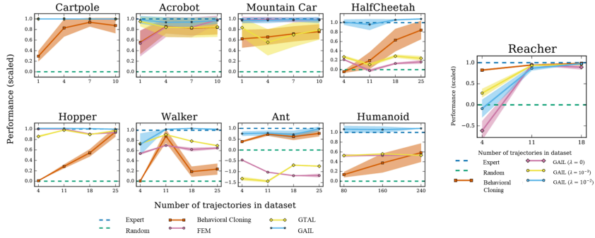
Figure 1.10: The performance comparison proposed in [78] is presented here. The y-axis shows the scaled reward, where the expert’s reward is set to 1 and the random baseline is set to 0. The IRL baselines FEM and GTAL refer to the IRL algorithm described in [80], but with different cost functions.
