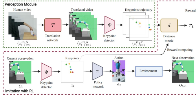
Figure 1.16: Architecture proposed by [38].
