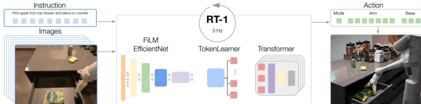
Figure 3.9: RT-1 Language-Conditioned Transformer based architecture proposed in [7].
