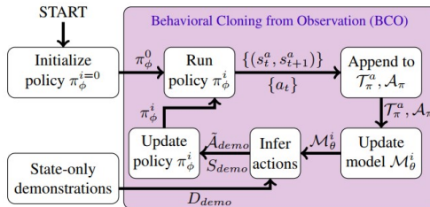
Figure 1.18: Representation of the learning procedure proposed by [97].
