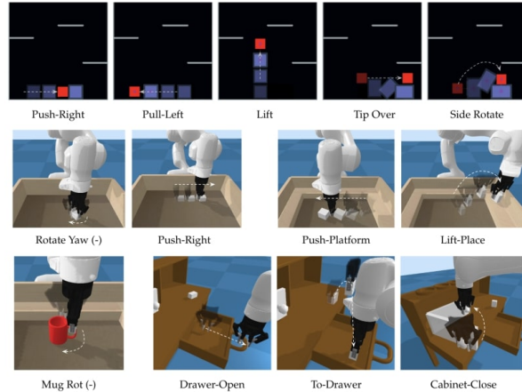
Figure 2.7: Testing scenarios and primitives proposed in [109]. (Top) Block2D Environment primitive examples. (Center) Block3D and Block3DPlatform primitive examples. (Bottom) The left image shows an example primitive in Mug3D-Platforms . The right three images show sample tasks from Playroom3D .
