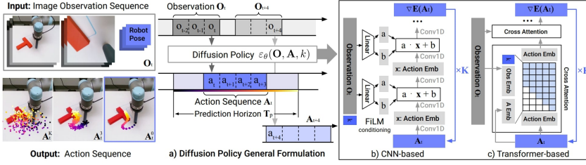
Figure 1.8: Architecture presented in [58]. (a) General formulation, at time step t , the policy inputs the latest T_o steps of observation data O_t and outputs T_a steps of actions A_t . (b) CNN-based Diffusion Policy, the observation feature O_t is conditioned using FiLM [62]. Starting with A_t^K from Gaussian noise, the noise-prediction network \epsilon_\theta iteratively subtracts noise to obtain the denoised action sequence A_t^0 . (c) Transformer-based Diffusion Policy, the observation embedding O_t is fed into a multi-head cross-attention layer within each decoder block, with causal attention applied to constrain each action embedding to attend only to itself and prior actions.
