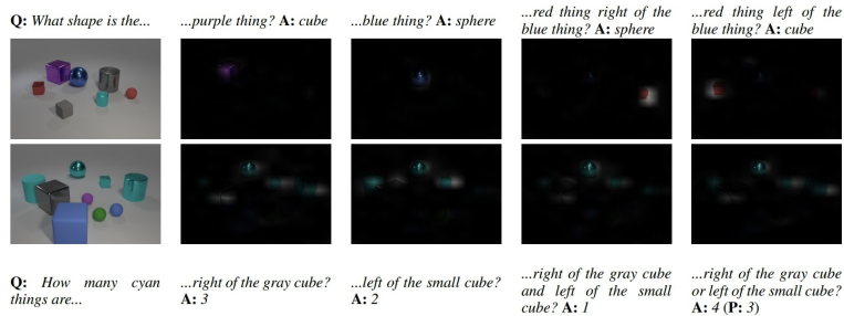
Figure 2.10: Visualizations of the distribution of locations used by the model for its globally max-pooled features, from which its final MLP makes predictions. FiLM correctly localizes the object referenced by the answer (top) or all objects referenced by the question (bottom). However, the localization is less accurate when the model provides an incorrect answer (rightmost bottom).
