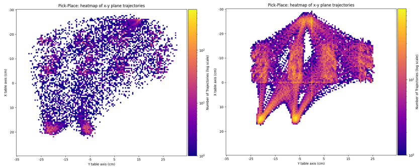
Figure 4.4: (Left) Trajectory distribution along the x-y axis of the real-world dataset. (Right) Trajectory distribution along the x-y axis of the simulated dataset, constrained to the same variations and number of trajectories as the real-world counterpart. It can be observed that the real-world dataset exhibits a much sparser and noisier distribution, due to the fact that the trajectories are collected via teleoperation.
