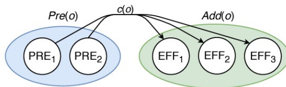
Figure 5.3: Example of nodes and edges definition in [147]. The hyper-edge represents an action that connects multiple nodes. The sending nodes are preconditions, while the receiver nodes are the effects.
