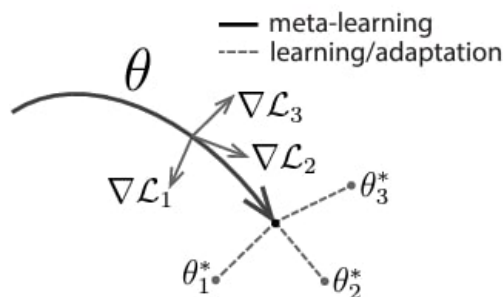
Figure 3.2: Diagram of MAML algorithm, which optimizes for a representation \theta that can quickly adapt to new tasks.
