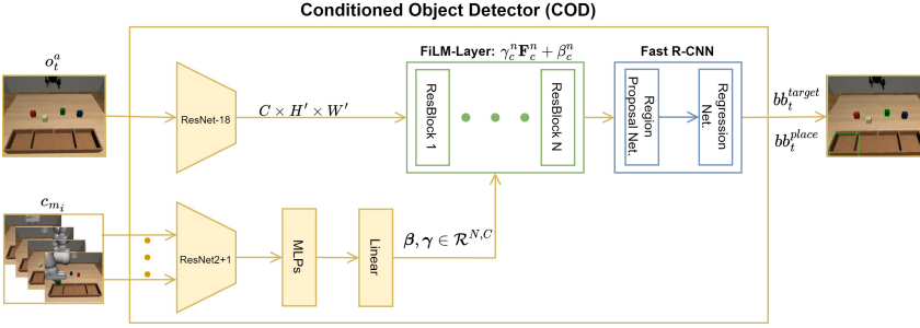
Figure 2.12: The proposed Conditioned Object Detector architecture takes as input the pair (o_t^a, c_{m_i}) , where o_t^a represents the agent observation and c_{m_i} represents the demonstration frames. The agent observation is encoded using ResNet-18, while the demonstration frames are encoded through ResNet2+1. The FiLM conditioning layer is employed to inject information from the command c_{m_i} into the feature maps extracted from the observation. Finally, Fast R-CNN generates the bounding boxes based on the conditioned input.
