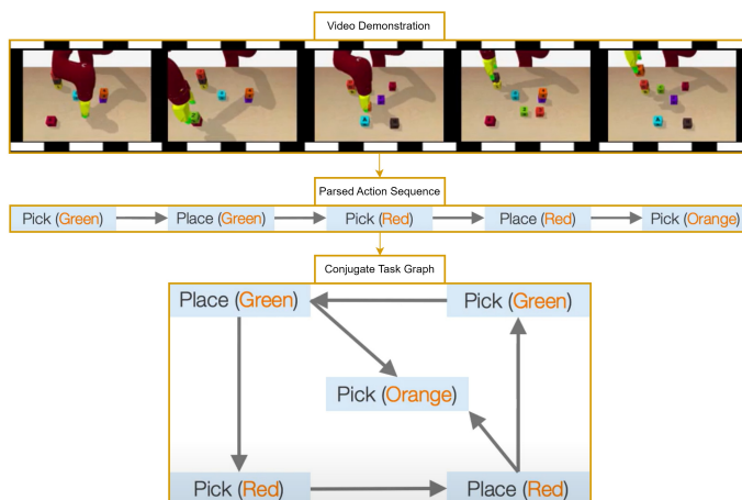
Figure 5.8: Conjugate Task Graph representation. Starting from the video demonstration, the sequence of actions is extracted and used to construct the initial graph. Then the complete Conjugate Task Graph is built by predicting the missing edges, which represents possible actions sequences observed in the training set.
