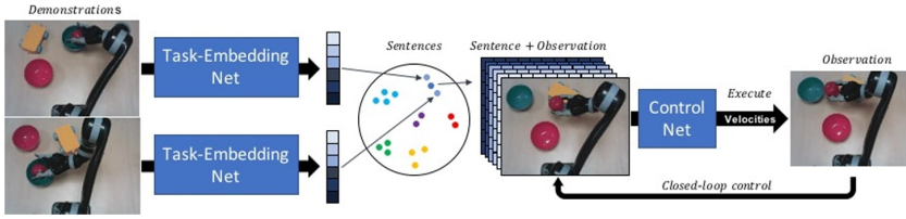
Figure 3.14: Architecture proposed in [16]. The Task Embedding Net generates the embedding representing the task to be performed given the goal image. The Control Net implements the policy, and takes in input the current observation and the tiled task embedding.
