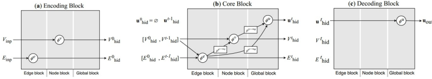
Figure 5.5: Computational flow of the STRIPS-HGN model [147], consisting of three main blocks: Encoding, Core, and Decoding. The Encoding Block generates initial hidden representations for both node and edge embeddings. The Core Block implements the message-passing mechanism, updating the hidden representations of nodes, edges, and global embeddings. Finally, the Decoding Block generates the output graph, where the global embedding represents the predicted heuristic value.
