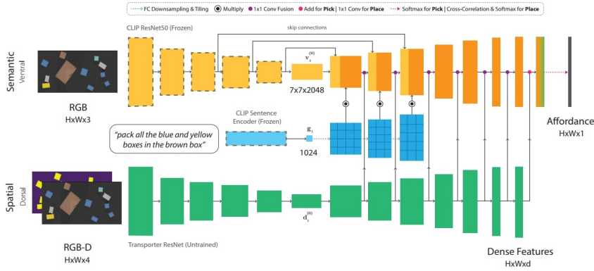
Figure 3.12: The Dual Stream architecture proposed in [135] consists of two parallel streams: a semantic stream and a spatial stream. The semantic stream utilizes a frozen CLIP ResNet50 to encode the RGB input, with the decoder layers conditioned by tiled language features from the CLIP sentence encoder. Meanwhile, the spatial stream encodes the RGB-D input, and its decoder layers are laterally fused with those of the semantic stream. The final output is a map of dense pixel-wise features, which is used to predict pick or place affordances.
