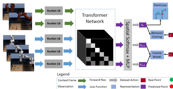
Figure 3.15: Transformer based architecture proposed in [6]. The Transformer network is used to create task-specific representation, given context and observation features computed with ResNet-18.
