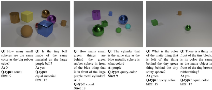
Figure 2.8: Example of Vision-Question Answering problem get from the CLEVR [116] dataset. It is possible to observe how for a given image multiple different questions can be done. As well as, questions covers different reasoning skills such as attribute identification, counting, comparison, multiple attention, and logical operations.
