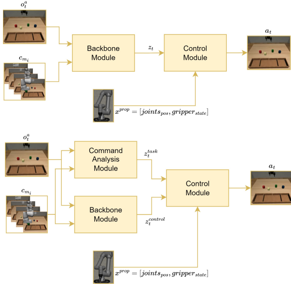
Figure 3.29: Proprioceptive information is integrated in both the end-to-end architecture (top) and the modular architecture (bottom). The proprioceptive vector, x^{prop} , is constructed from the robot’s six continuous joint positions and the binary gripper state.
