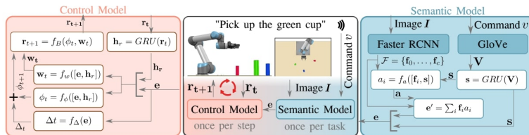
Figure 3.5: Architecture proposed in [9]. The Semantic Model takes in input the image I and the command v , generating a command conditioned embedding e . The Control Module receives in input the embedding e and the current robot state r_t and produces the next control signal.
