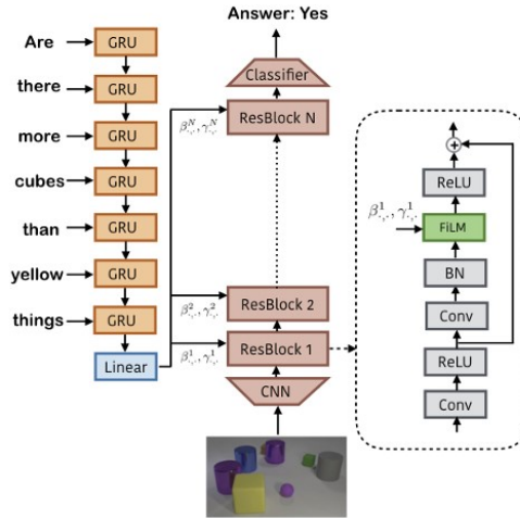
Figure 2.9: Proposed integration of the FiLM conditioning layer. Here, the Linear Modulation is applied to modify the activation maps of the ResNet blocks, while a linear layer generates the modulation coefficients \beta and \gamma based on the embedding derived from the textual prompt. This enables the model to conditionally adjust the activation maps according to the context provided by the input query.
