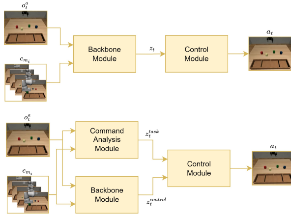
Figure 3.20: (Upper) General end-to-end architecture, where the Backbone Module takes as input both the agent observation and the command. It generates an embedding z_t that must contain information related to both the command and the control. (Bottom) In the modular architecture, there are two backbone modules: the Command Analysis Module , which generates the task-embedding z_t^{task} , and the Backbone Module , which is trained to generate only the control-embedding z_t^{control} .
