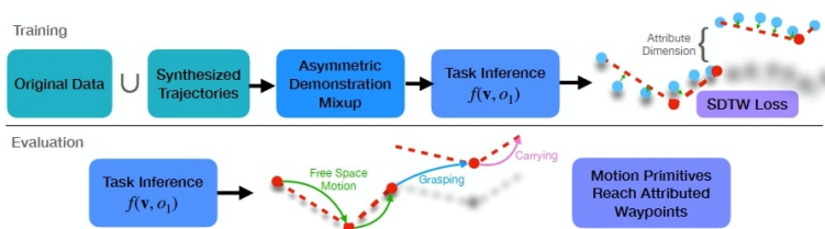
Figure 3.19: AWDA framework proposed in [26]. The task inference network f(v, o) predicts a sequence of attributed waypoints (red dots) that are achieved by hand-defined motion primitives. The original data are augmented with free-space motion trajectories and asymmetric demonstration mixup in order to reduce the correlation between tasks and task content.
