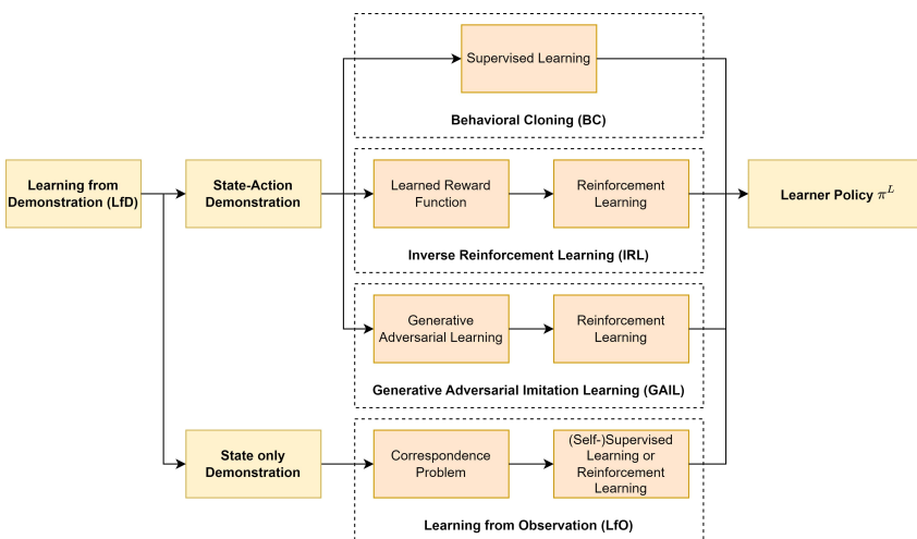
Figure 1.4: Taxonomy of LfD methods, divided based on type of demonstration and the learning algorithm used to learn the learner policy \pi^L .
