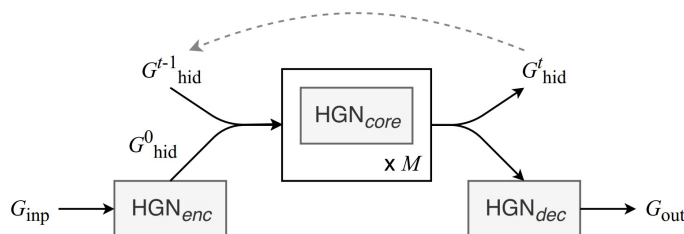
Figure 5.4: Architecture of the STRIPS-HGN model [147]. The model is composed of three main components: the encoder, the hyper-graph network, and the decoder. The encoder processes the input graph, generating a first hidden graph representation. The HGN implements the message passing mechanism, updating the hidden graph representation. The decoder generates the output graph, which global value represents the predicted heuristic.
