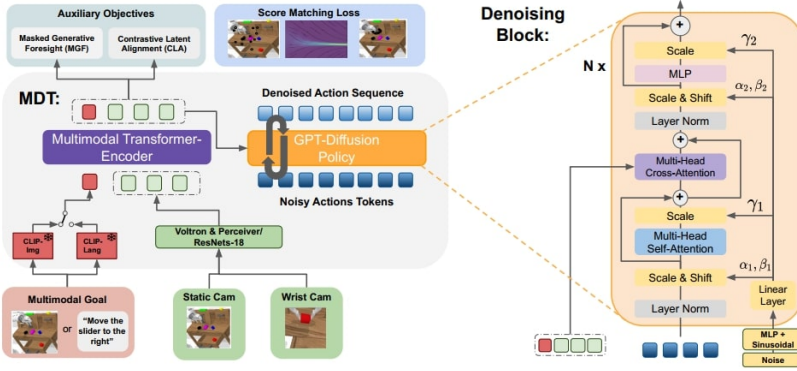
Figure 3.11: The Multimodal Diffusion Transformer (MDT) architecture proposed in [134].
