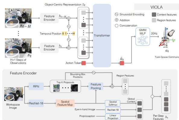
Figure 2.4: The VIOLA architecture proposed in [110]. (Top) The overall control architecture is based on a Transformer module that processes a stack of per-step features h_t , obtained from the Feature Encoder, to generate a final action embedding, which is then input into a GMM policy. (Bottom) The Feature Encoder builds both local and global features. Local features correspond to regions of interest extracted by the RPN. Global features are obtained by processing the workspace image, the image from the camera on the gripper, and proprioceptive information.
