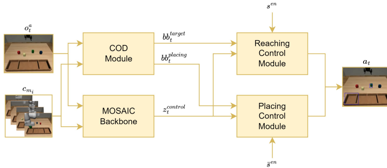
Figure 3.22: Proposed Double-Control Module Architecture. In this architecture, the Control Module is split into two distinct modules, each responsible for learning a specific primitive: the reaching primitive and the placing primitive. The first module takes as input the bounding box corresponding to the target object ( bb_t^{target} ), while the second module receives the bounding box related to the final placing location ( bb_t^{placing} ). This separation allows for specialized control during both the reaching and placing phases.
