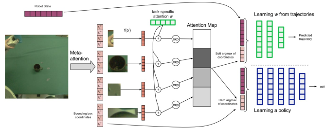
Figure 2.1: Robotic vision framework proposed in [107]. The framework is divided into different stages: Meta-Attention : Generates object proposals from an input image, trained on an object detection dataset, and shared across tasks; Task-Specific Attention : Focuses on relevant objects for a task using the meta-attention’s semantic features; Soft Attention : Distributes attention as probabilities over object proposals using a Boltzmann distribution; Movement Prediction Network : Combines attended object information with the robot’s state to predict the next action.
