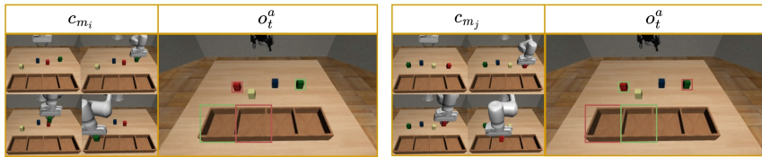
Figure 2.11: Example of bounding-boxes assignment, where green boxes refer to target object and placing location while red boxed refers to no-target and no-target-place. (Left) The demonstrator manipulates the green box, placing it into the first bin. (Right) The demonstrator manipulates the red box, placing it into the second bin. Note, how for a given agent environment state, the semantic attribute between objects changes.
