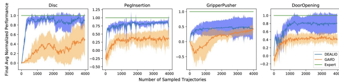
(b) Performance of DEALIO [98] compared against GAfO [96], with respect to the number of trajectories sampled during the learning process.
