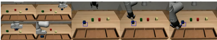
Figure 3.27: Example of an unsuccessful Pick-Place operation using the “no-bb after pick” variant. In this scenario, the robot successfully reaches the target box based on the predicted bounding box (blue). However, the single-control module prematurely predicts the closing command, preventing the robot from correctly picking up the object.
