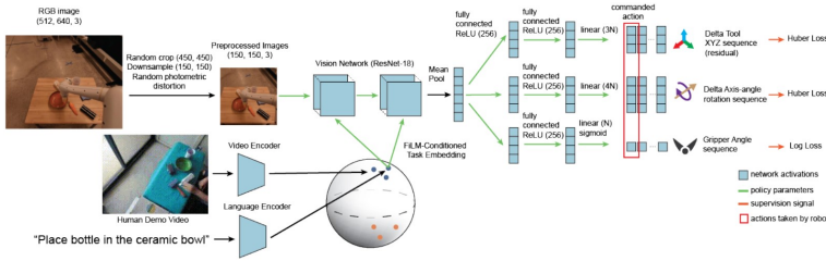
Figure 3.7: Architecture proposed in [13]. Here, the Task Embedding is injected directly in the Feature Maps generated by the ResNet-18.
