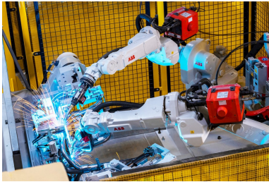
(a) Robots involved in arc welding operation.
