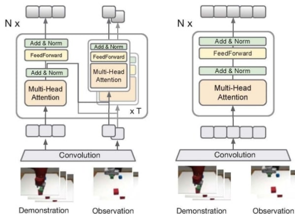
Figure 3.17: (Left) The TOSIL architecture, as proposed in [6]. (Right) The MOSAIC architecture, as introduced in [8]. In the MOSAIC architecture, the original encoder-decoder Transformer architecture has been replaced with an encoder-only architecture featuring self-attention modules.
