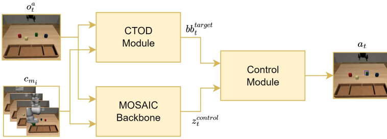
Figure 3.21: Proposed Single-Control Module Architecture. In contrast to the general architecture described in Figure 3.20, the Command Analysis module is replaced by the CTOD module, which generates the bounding box related to the target object. The chosen backbone is the MOSAIC architecture [8]. The control module is now informed by both low-level positional information ( bb_t^{target} ) and a control-oriented embedding ( z_t^{control} ), enabling it to make more informed decisions.
