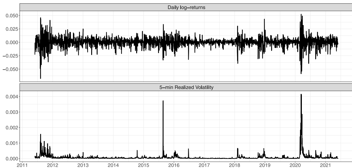
Fig. 1. Daily log-returns (top panel) and 5-minute Realized Volatility (bottom panel) of the S&P 500 index for the full sample period June 01, 2011–June 01, 2021.
