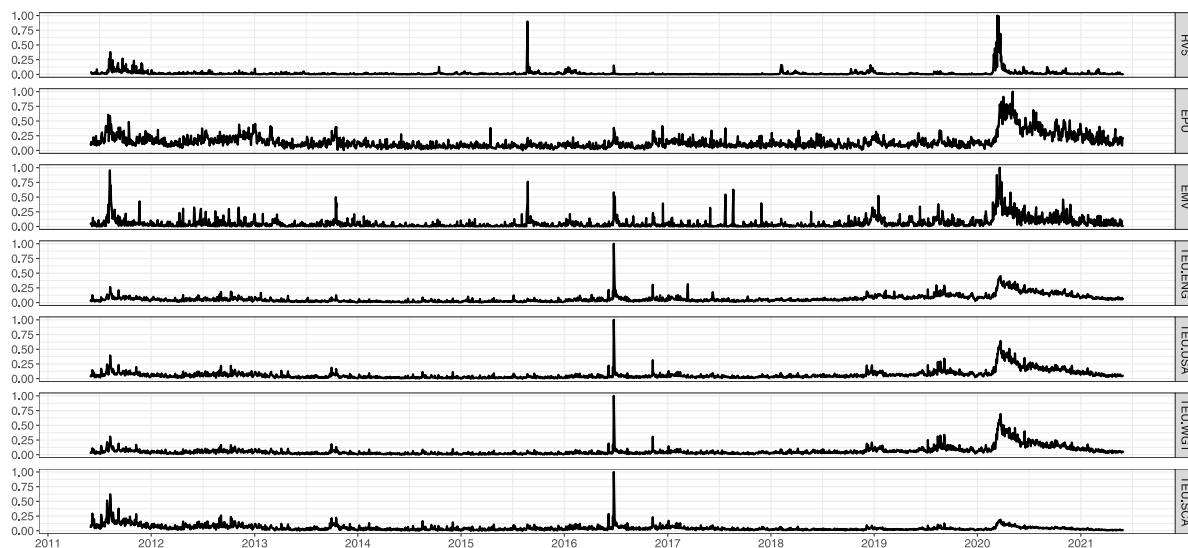
Fig. 2. 5-min Realized Volatility and uncertainty indices. Time series of all normalized explanatory variables for the full sample period June 01, 2011–June 01, 2021.
