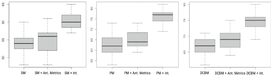
Fig. 1 Overview of the value of F-measure among the models. Note that the starting value of the y-axis is different based on the performance of the models
