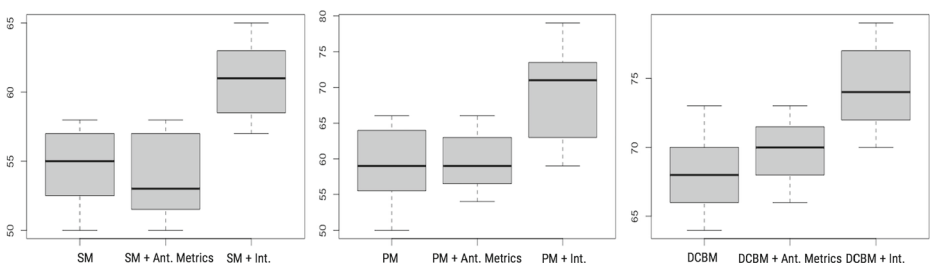
Fig. 2 Overview of the value of AUC-ROC among the models. Note that the starting value of the y-axis is different based on the performance of the models
