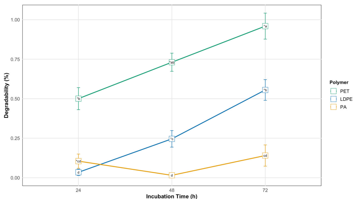
Figure 3. Ruminal degradability (%) of PET (polyethylene terephthalate), LDPE (low-density polyethylene), and PA (polyamide) polymers during in vitro incubation with buffered rumen fluid (incubation times: 24, 48, and 72 h). To test whether degradability was significantly greater than 0%, a Wilcoxon test was applied (* = p -value < 0.05). To compare degradability differences among the three polymers across incubation times, a Kruskal–Wallis test was applied (a–d = p -value < 0.05).
