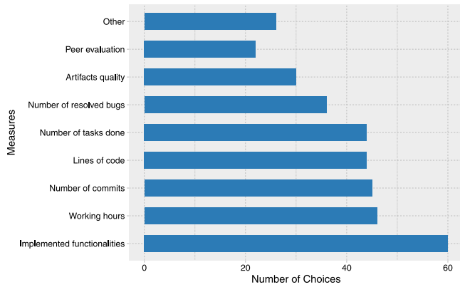
Fig. 7. Productivity measures.
