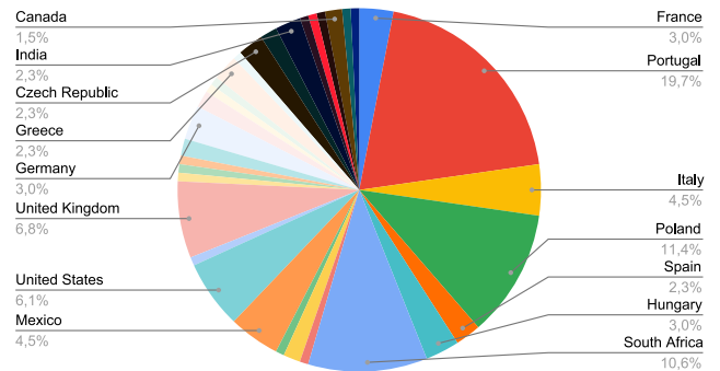
Fig. 6. Participants Nationalities.
