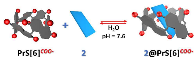
Fig. 2 Cartoon representation of the complexation equilibrium of prism[6]arene \text{PrS[6]}^{\text{COO}^-} with aniline derivatives at 25 °C in a buffered aqueous solution (pH 7.6).
