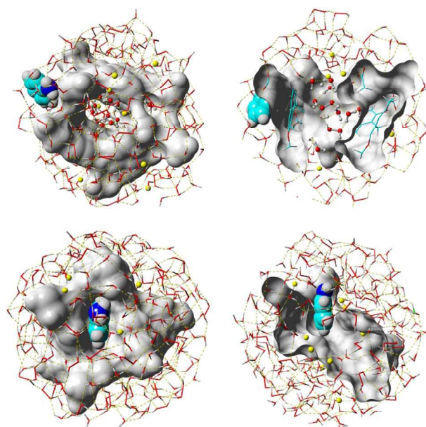
Fig. 5 Top (up left) and side section (up right) views of the 2a + \text{PrS[6]}^{\text{COONa}} inside the spherical nanoreactor; top (bottom left) and side section (bottom right) views of the 2a + \text{PrS[6]}^{\text{COONa}} inside the spherical nanoreactor. Compound 2a and \text{Na}^+ ions are represented as balls (in the upper right, also \text{H}_2\text{O} and \text{H}_2\text{O}_2 molecules within the cavity), \text{H}_2\text{O} and \text{H}_2\text{O}_2 molecules as stick lines, and \text{PrS[6]}^{\text{COONa}} is rendered as a molecular surface. Dashed lines represent hydrogen bonds.
