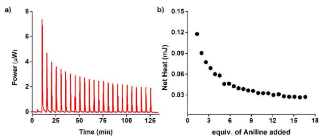
Fig. 3 (a) ITC titration of \text{PrS[6]}^{\text{COO}^-} (0.92 mM) with aniline 2a (up to 16.6 equiv.) at 25 °C and pH 7.6; (b) integrated net heat curve.
