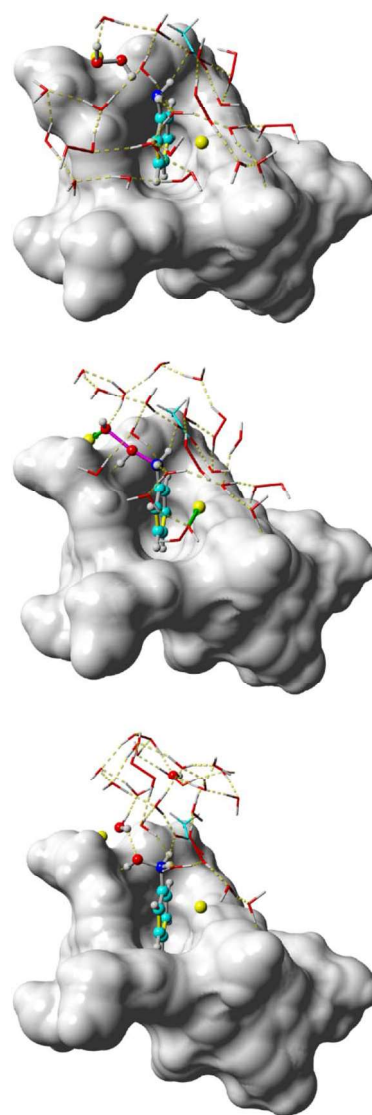
Fig. 6 Detail of 2a@PrS[6]^{COONa} (top), 2a@PrS[6]^{COONa}\cdot TS (middle) and 2a@PrS[6]^{COONa}\cdot P (down). Compound 2a , one interacting \text{H}_2\text{O}_2 molecule, and \text{Na}^+ ions are represented as balls, \text{H}_2\text{O} and \text{H}_2\text{O}_2 molecules as stick lines, and \text{PrS}[6]^{\text{COO}^-} is rendered as a molecular surface. Dashed lines represent hydrogen bonds.
