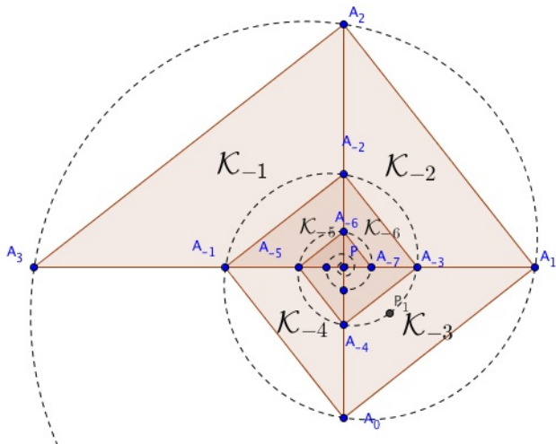
FIGURE 1.3. \mathcal{K}_{n-1} \cup \mathcal{K}_{n-2} , is congruent to \mathcal{K}_n
