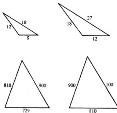
FIGURE 2.1. Pairs of almost congruent triangles with integer sides. Each of them is a continue triangle
