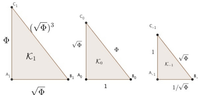
FIGURE 1.2. Examples of Kepler triangles
