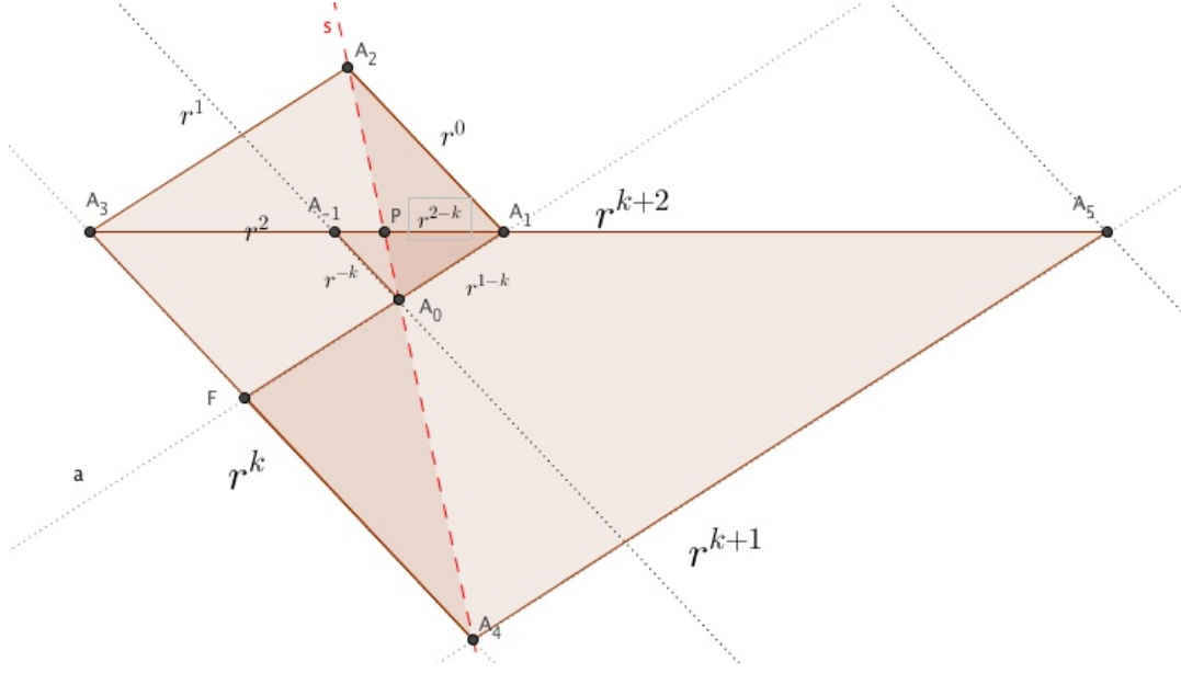
FIGURE 3.2. The Pole of the (r, k) -male spiral
