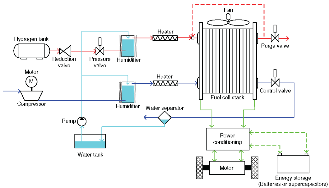
Figure 4: Schematic of a fuel cell system.
