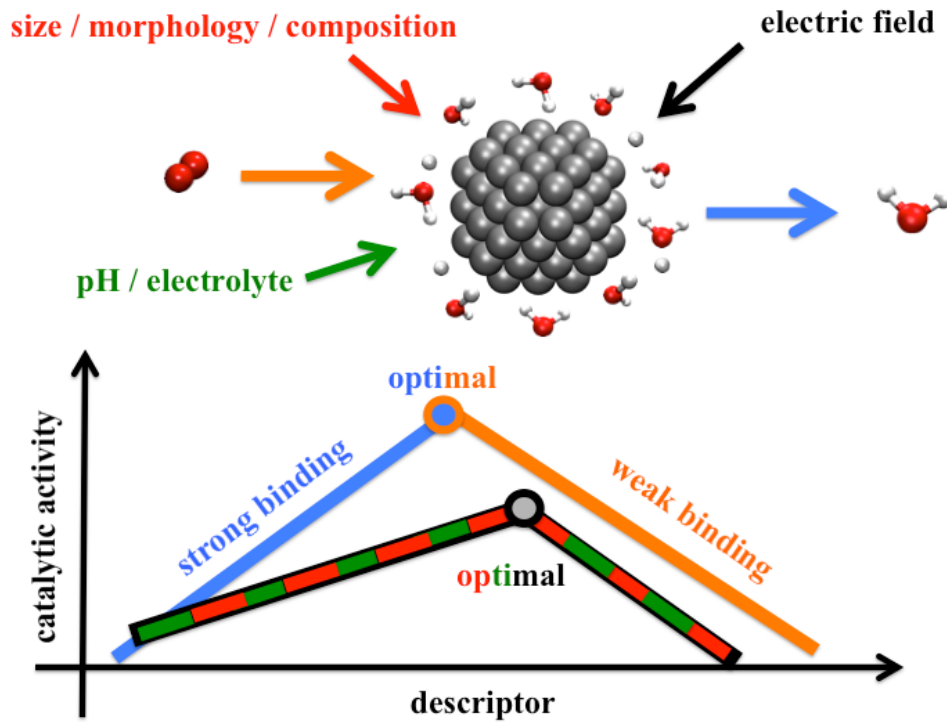
Figure 2: Schematics of Sabatier-type volcano plots. The blue and orange lines represent the usual approach based only on the adsorption strength of the adsorbates to the catalyst surface. The black-green-red lines represent the real situation in which several other effects (catalyst composition and morphology, environment) are taken into account in addition to binding in order to provide realistic predictions.
