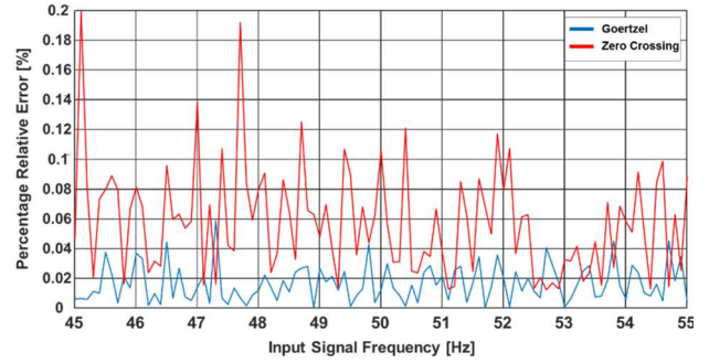
Figure 7 Percentage relative error with Goertzel and zero-crossing techniques.
