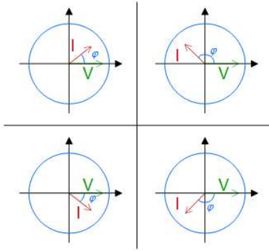
Figure 6 Quadrants graphical representation of power flow directions.
