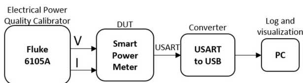
Figure 9 Functional block diagram of experimental setup.
