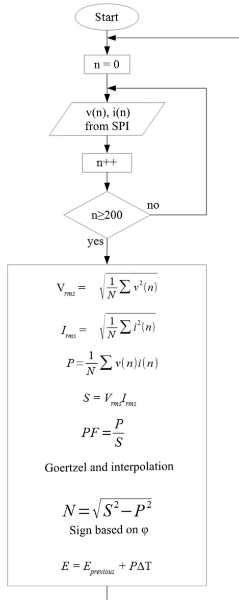
Figure 8 Flowchart of the data acquisition and processing firmware.
