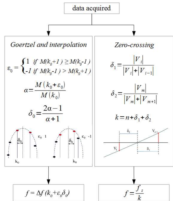
Figure 5 Block diagram for comparison of the two algorithms implemented.
