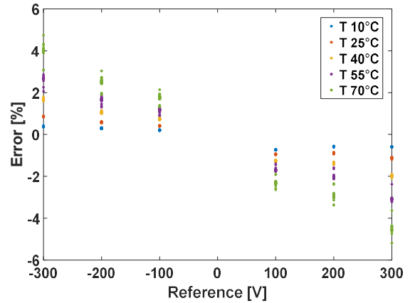
Figure 10 Error versus voltage at different temperatures
