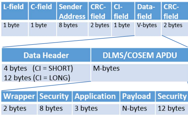
Figure 2 The frame of the wM-Bus.
