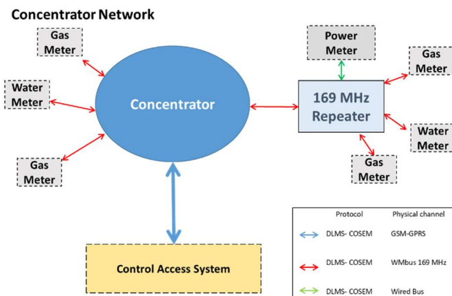
Figure 3 Concentrator Network.
