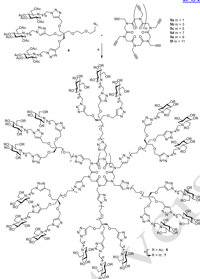
Scheme 1. Reagents and conditions: Synthesis of DNJ clusters 7 : (a) \text{CuSO}_4 \cdot 5\text{H}_2\text{O} cat., sodium ascorbate, DMF/ \text{H}_2\text{O} (5:1), MW, 80^\circ\text{C} or 90^\circ\text{C} ; 6a ( m = 1 ) 75%; 6b ( m = 3 ) 73%; 6c ( m = 5 ) 53%; 6d ( m = 7 ) 70%; 6e ( m = 9 ) 77%; 6f ( m = 11 ) 32%. (b) Amberlite ( \text{OH}^- ), \text{MeOH}/\text{H}_2\text{O} (1:1), 40^\circ\text{C} ; 7a ( m = 1 ) 88%; 7b ( m = 3 ) 77%; 7c ( m = 5 ) quant.; 7d ( m = 7 ) 57%; 7e ( m = 9 ) 81%; 7f ( m = 11 ) 85%
