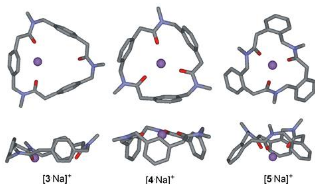
Fig. 5 Minimum energy structures of \text{Na}^+ complexes of compounds 3–5 (top and side views). For simplicity's sake, the N -linked side chain has been modelled as -\text{CH}_3 . Hydrogen atoms have been omitted for clarity. Atom type: C grey, N light blue, O red, \text{Na}^+ blue.
