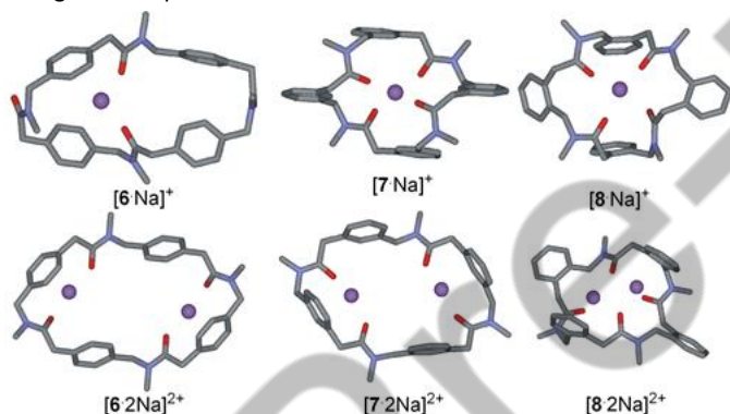
Fig. 6 Minimum energy structures of \text{Na}^+ complexes of compounds 6–8 with one or two coordinated \text{Na}^+ . For simplicity's sake, the N -linked side chain has been modelled as -\text{CH}_3 . Hydrogen atoms have been omitted for clarity. Atom type: C grey, N light blue, O red, \text{Na}^+ blue.
