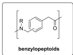
Fig. 3 Structural unit of “benzylpeptoids”.
