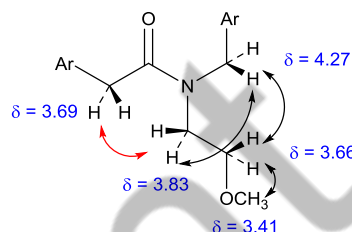
Fig. 8 ROE effects (600 MHz) in the case of [\mathbf{4}\cdot\text{Na}][\text{TFPB}] . In red the key cross correlation inferring the trans peptoid conformation.
