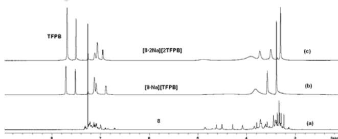
Fig. 9 ^1\text{H} NMR spectra of free 8 (a) ( \text{CDCl}_3 , solution, 298 K, [\mathbf{8}] = 4.0 mM, 600 MHz), in the presence of 1.0 (b) and 2.0 equivalents (c) of NaTFPB.
