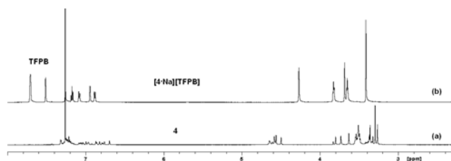
Fig. 7 ^1\text{H} NMR spectra of free 4 (a) ( \text{CDCl}_3 solution, 298 K, [\mathbf{4}] = 4.0 mM, 600 MHz) and (b) in the presence of 1.0 equivalent of NaTFPB.
