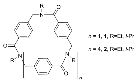
Fig. 2 para -Series of properly N -substituted arylopeptoids.
