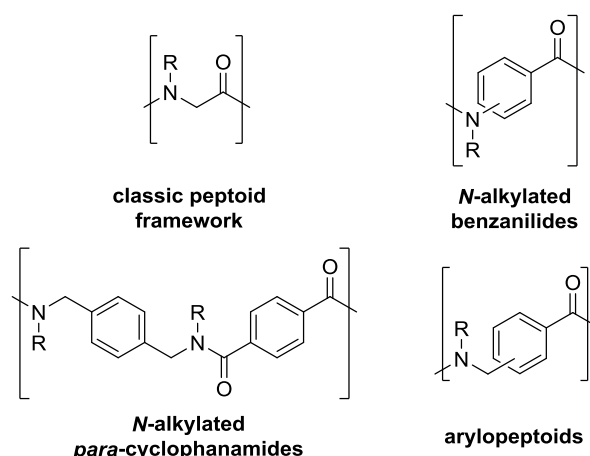
Fig. 1 Peptoids and tertiary oligoamides with aromatic backbones.
