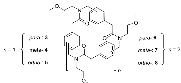
Fig. 4 Structures of cyclic benzylpeptoids 3–8 ( i.e. : cyclic oligomeric N -substituted aminomethyl phenylacetamides).
