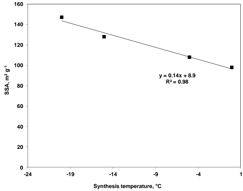
Fig. 5 Trend of NDC specific surface area (m 2 g -1 ) as a function of sol-gel synthesis reaction temperature
