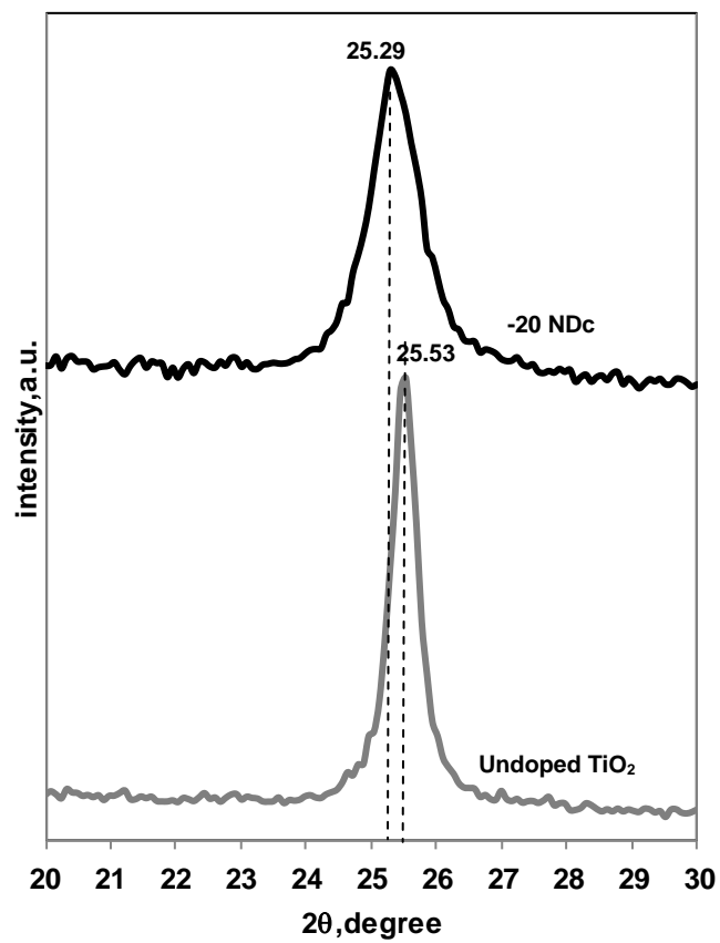
Fig. 4 XRD patterns of NDc of undoped TiO 2 and -20 NDc sample in the range 20-30 degree
