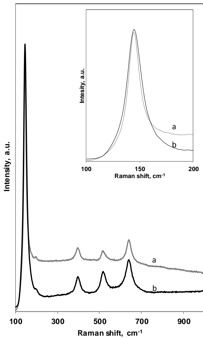
Fig. 1 Raman spectra of (a) N-TiO 2 synthesized by sol-gel method at 0°C and (b) ONDc synthesized by sol-gel method at 0°C using surface-active agent (Triton X-100); Raman shift of E g modes in the range 110-200 cm -1 (insert)
